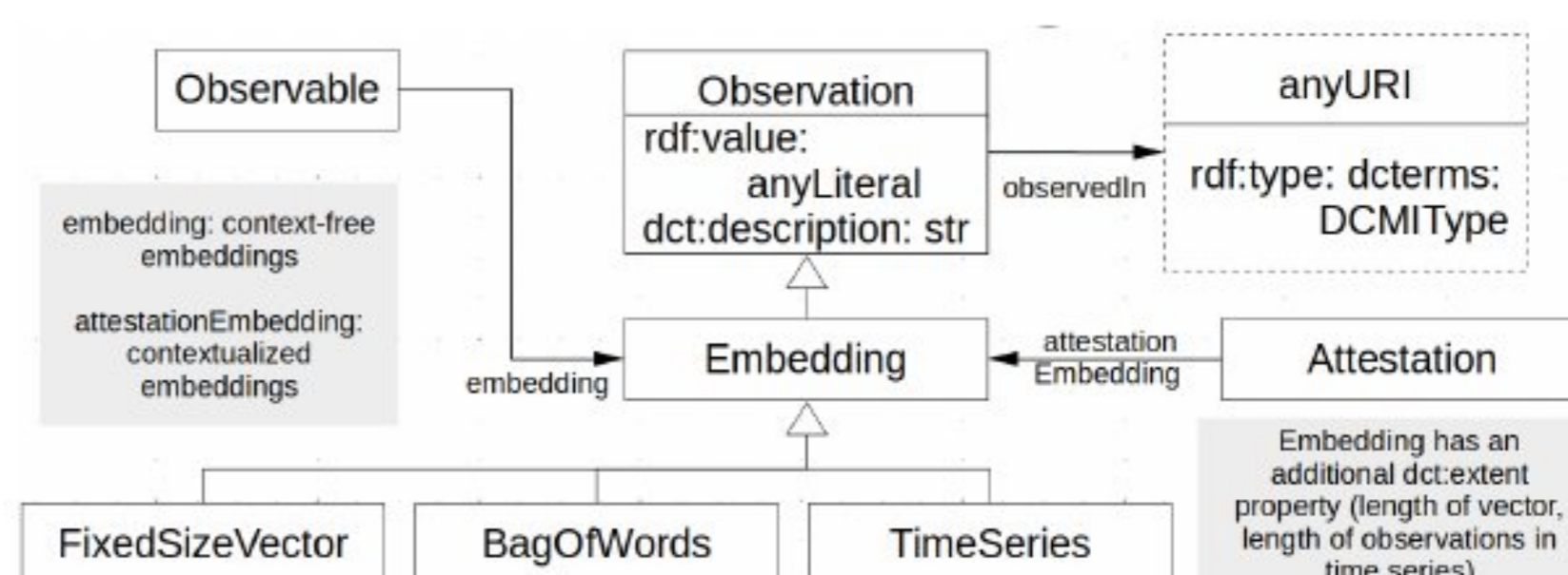
Figure 4: Embeddings in OntoLex-FrAC
