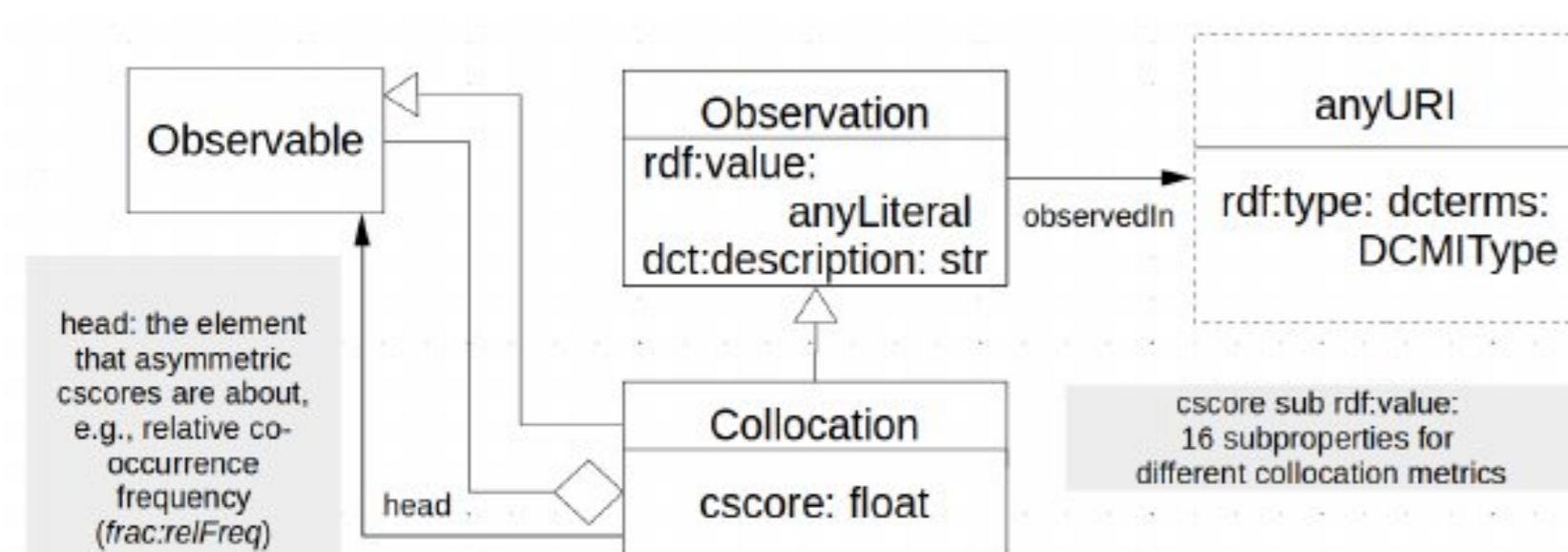
Figure 6: Collocations in OntoLex-FrAC
