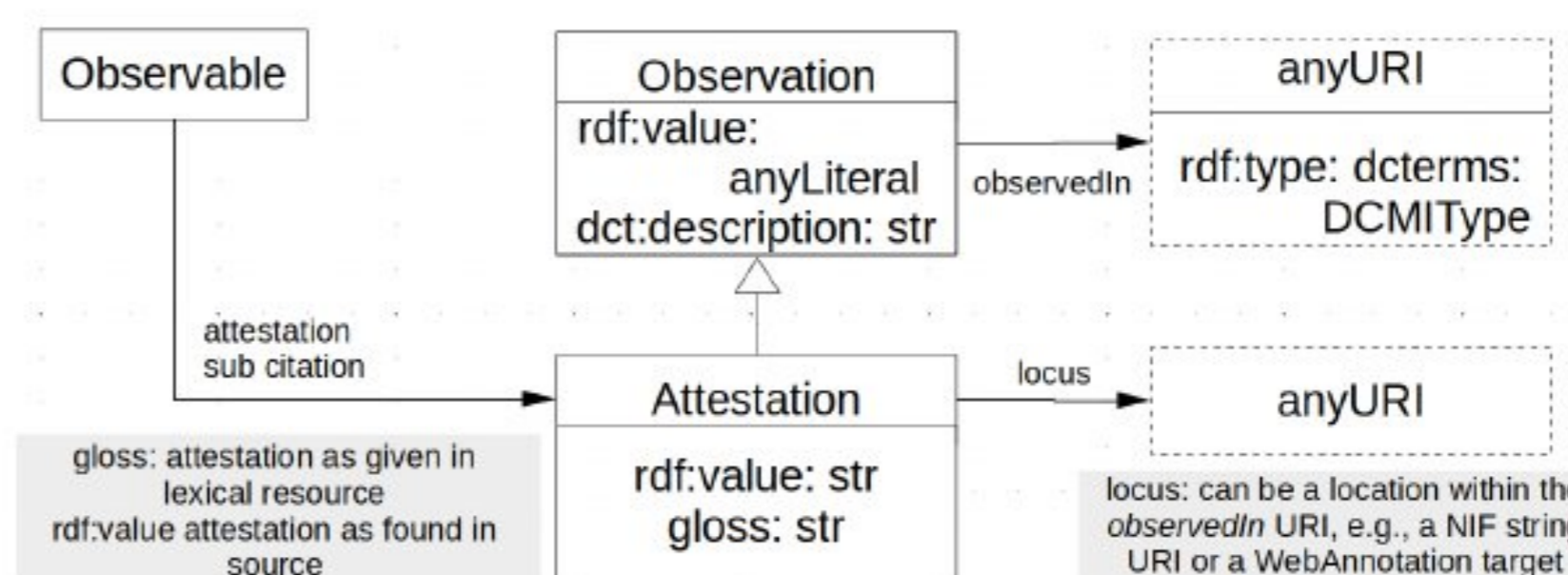
Figure 3: Attestations in OntoLex-FrAC
