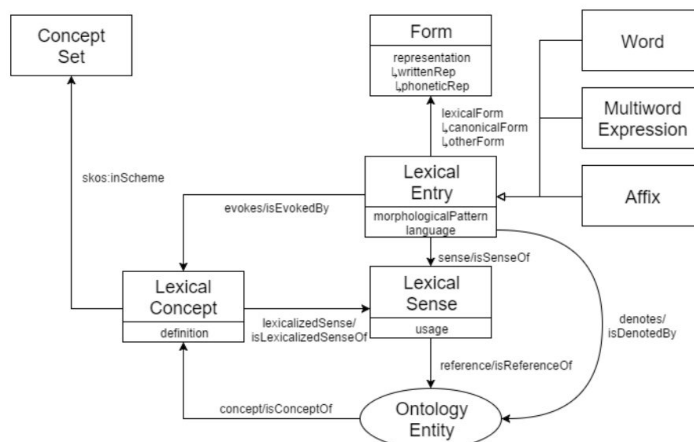
Figure 1: OntoLex-Lemon, the OntoLex core vocabulary, https://www.w3.org/2016/05/ontolex/#core
