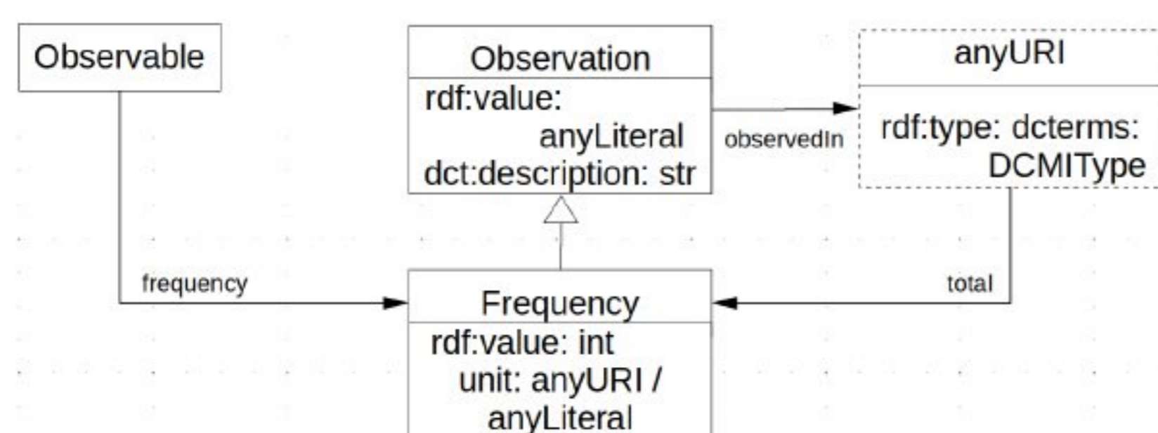
Figure 2: Frequency in OntoLex-FrAC
