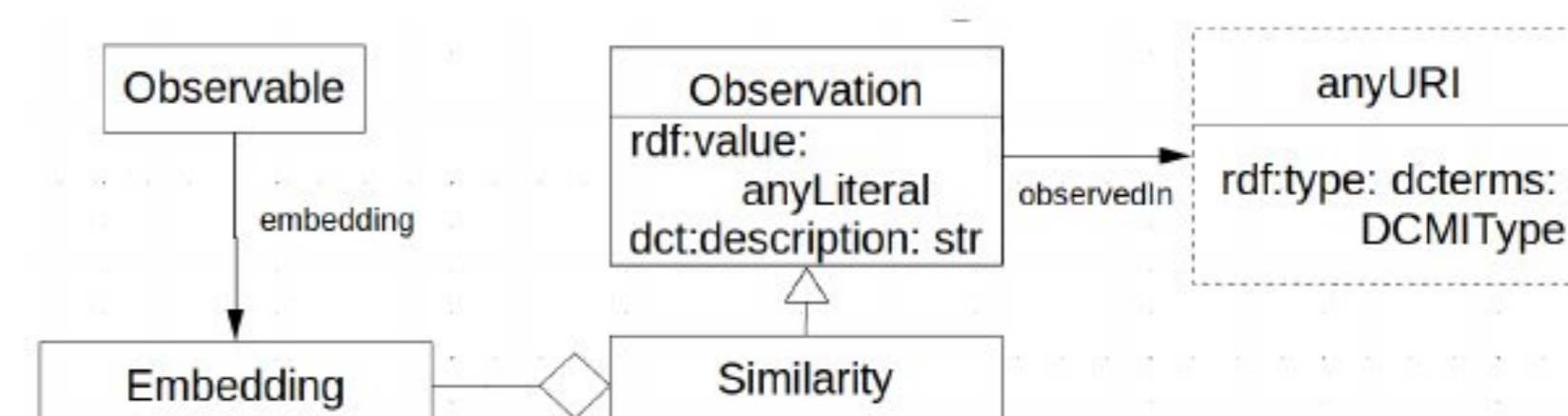
Figure 5: Distributional similarity in OntoLex-FrAC
