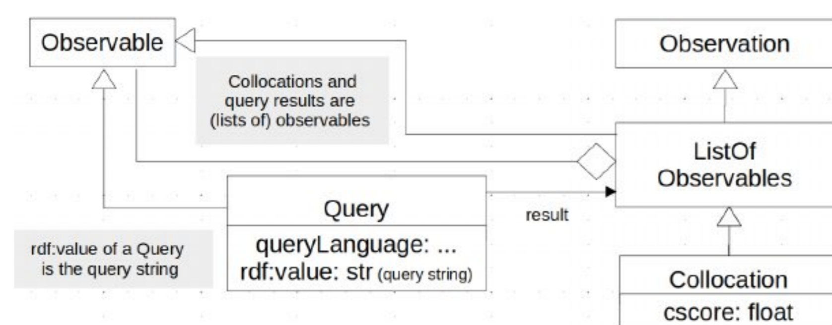
Figure 7: Proposed query extension
