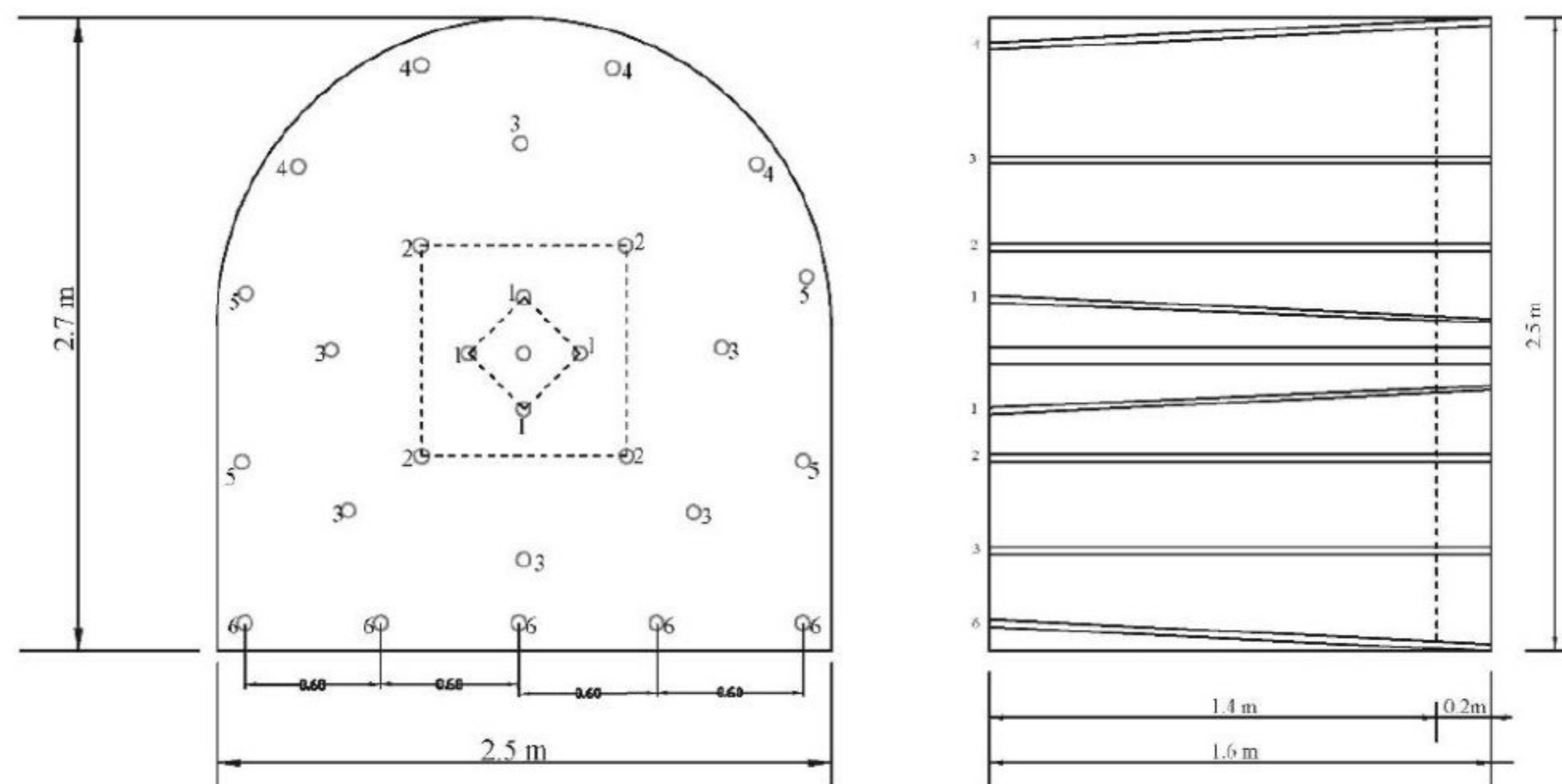
Figure 1 Blasting pattern used in Lece mine
