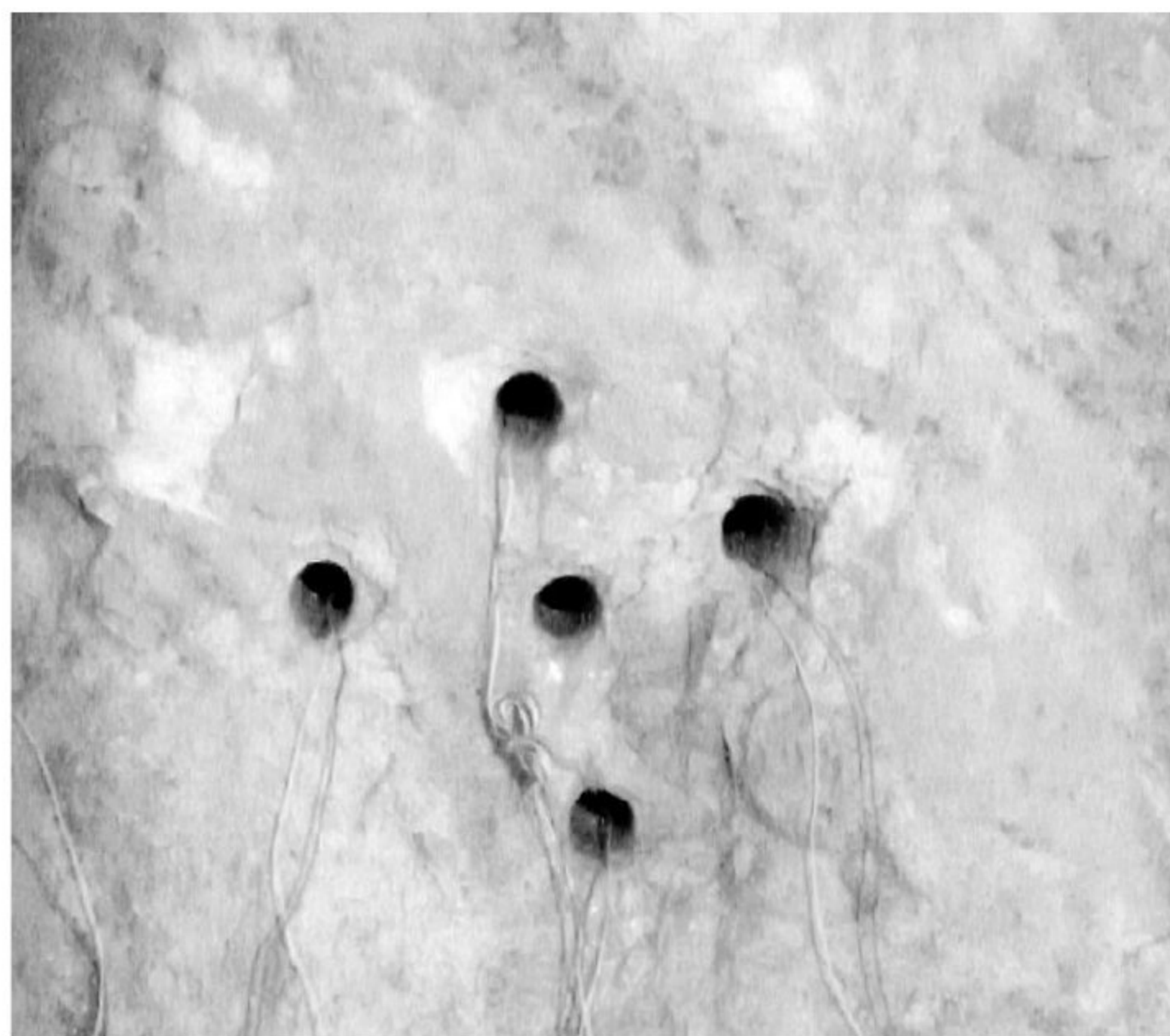
Figure 6 Drilled and charged cut prepared for blasting
