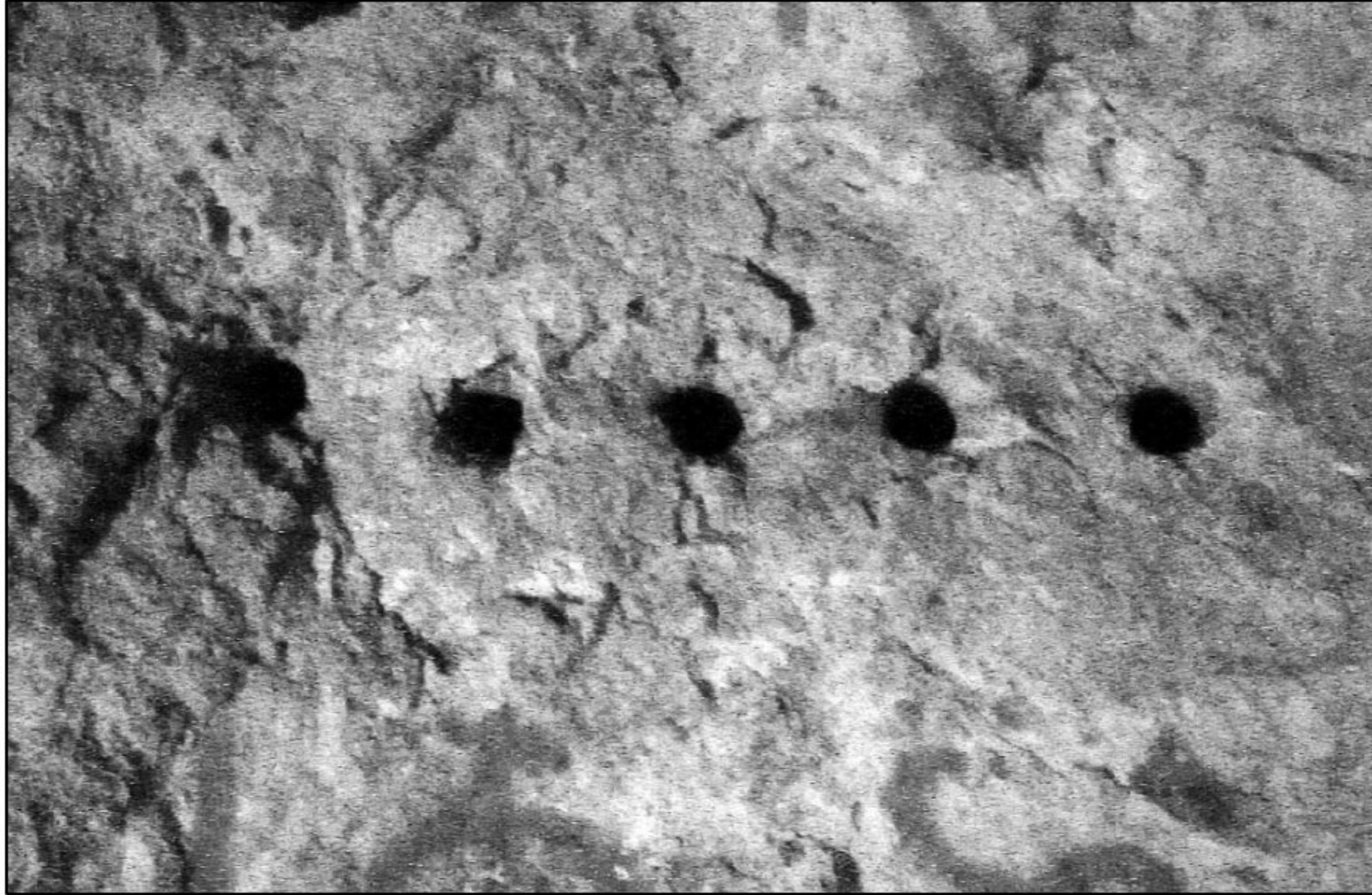
Figure 2 Line cut drilling pattern
