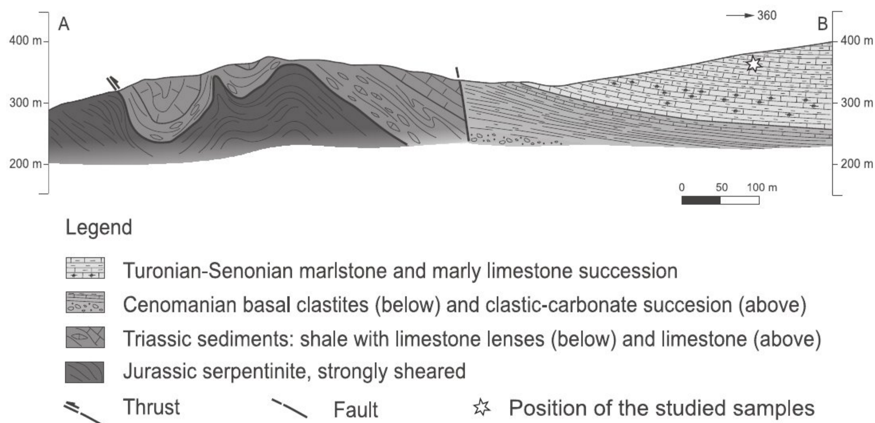
Figure 3: A Simplified geological profile in Brežde village.
