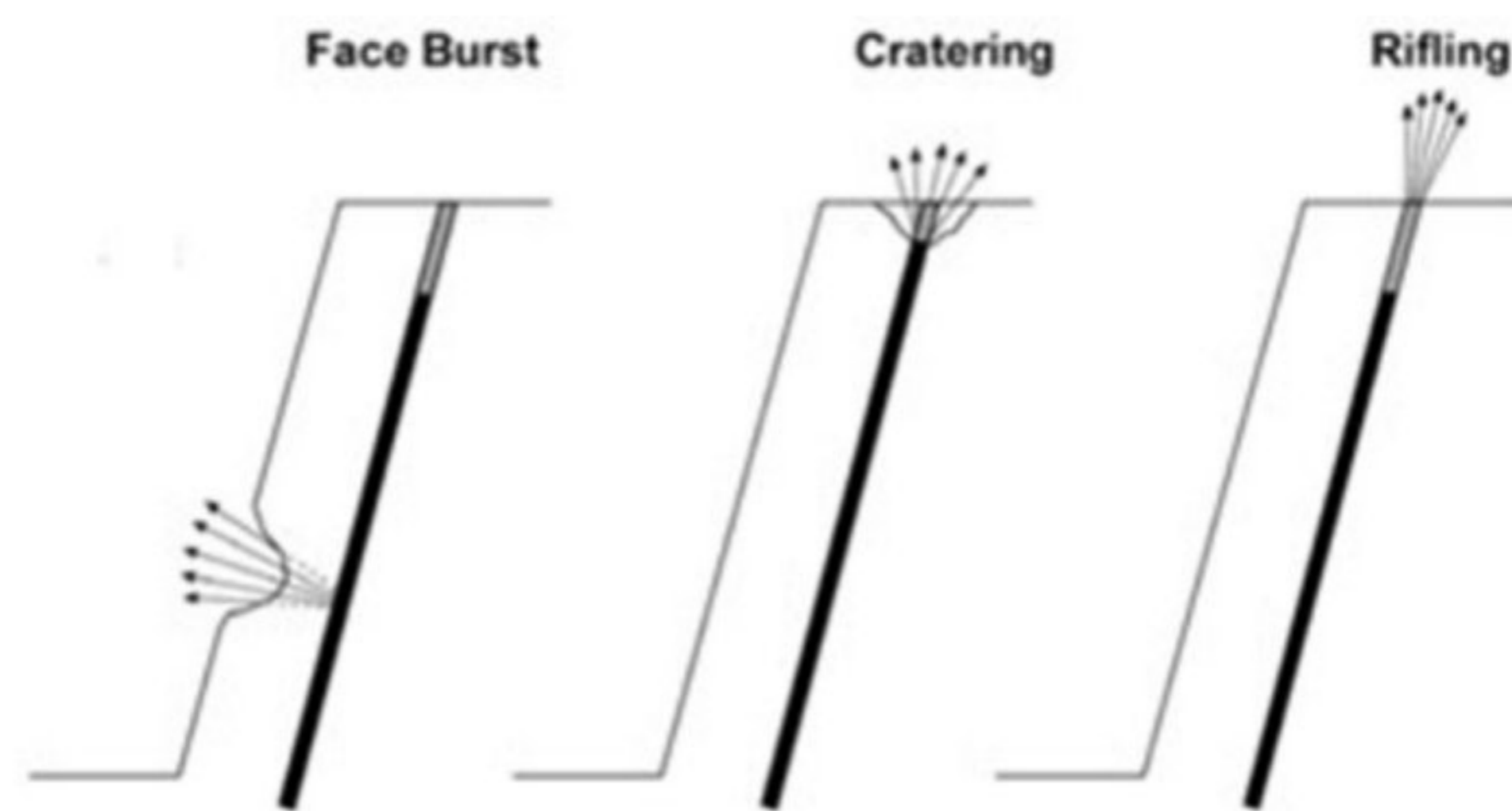
Figure 7 The three key mechanisms of flyrock ( https://www.o-pitblast.com/ )
