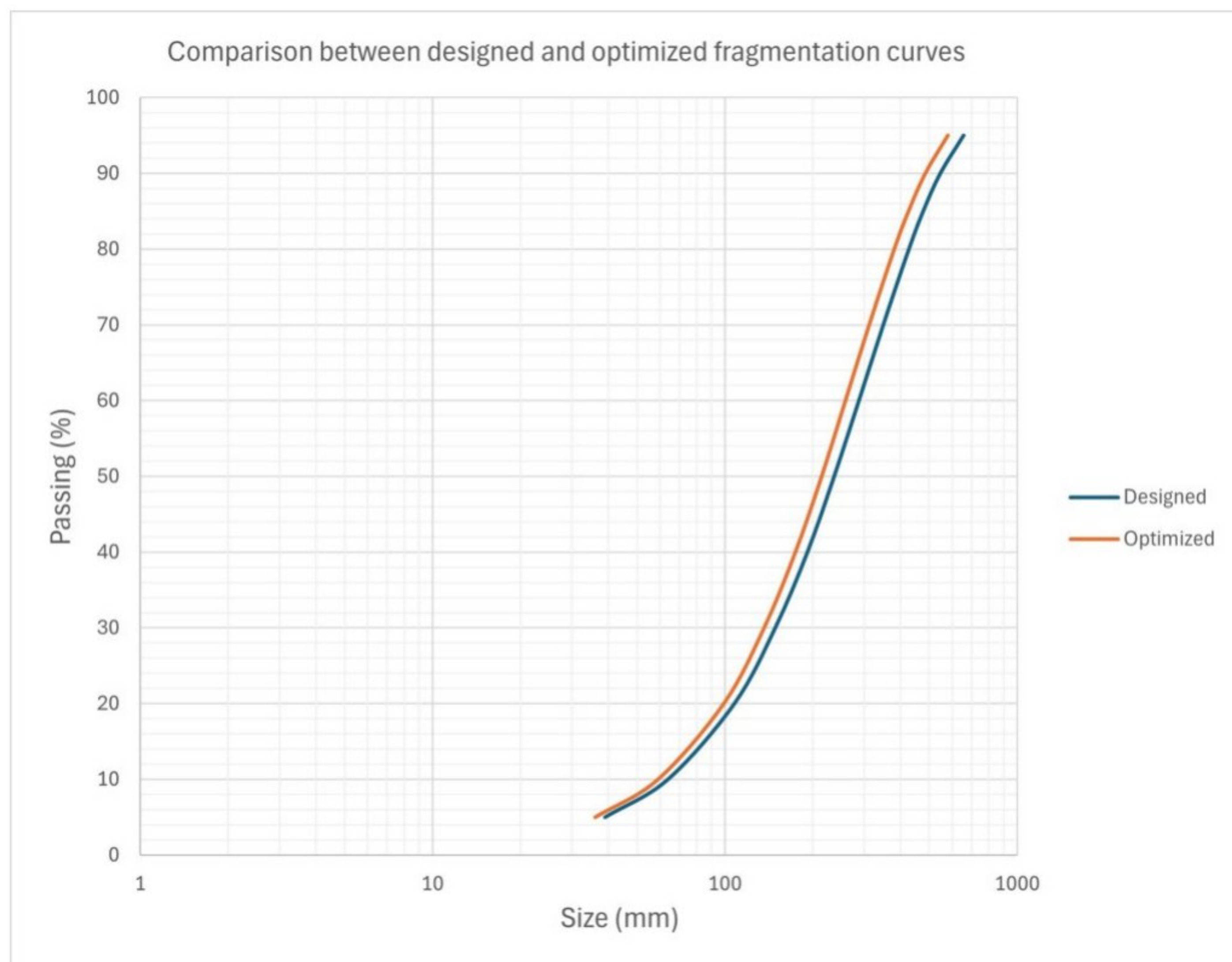
Figure 12 Comparison between designed and optimized fragmentation curves
