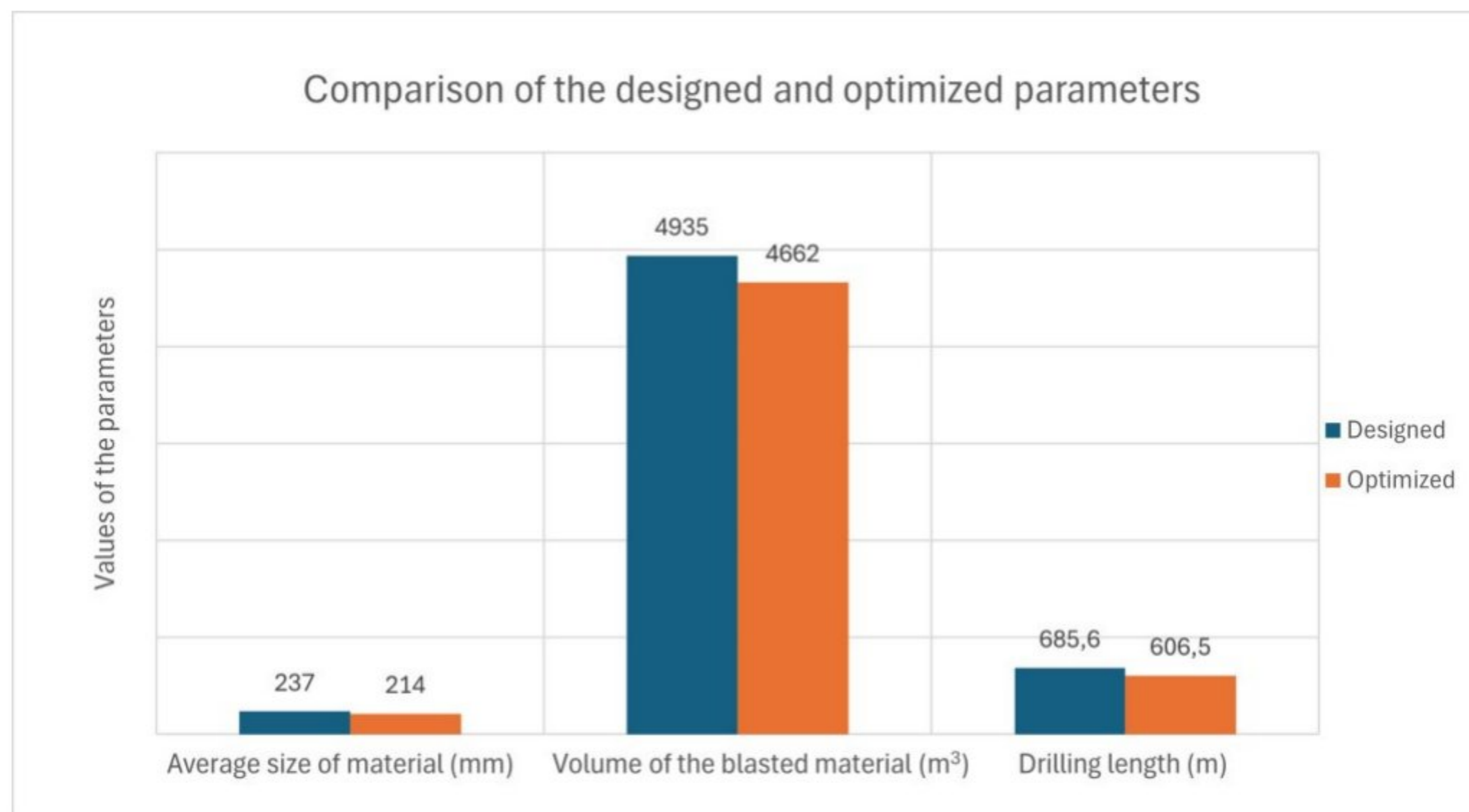
Figure 13 Comparison between designed and optimized parameters
