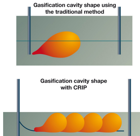
Figure 4. Schematic of CRIP process compared to traditional methods [8]
